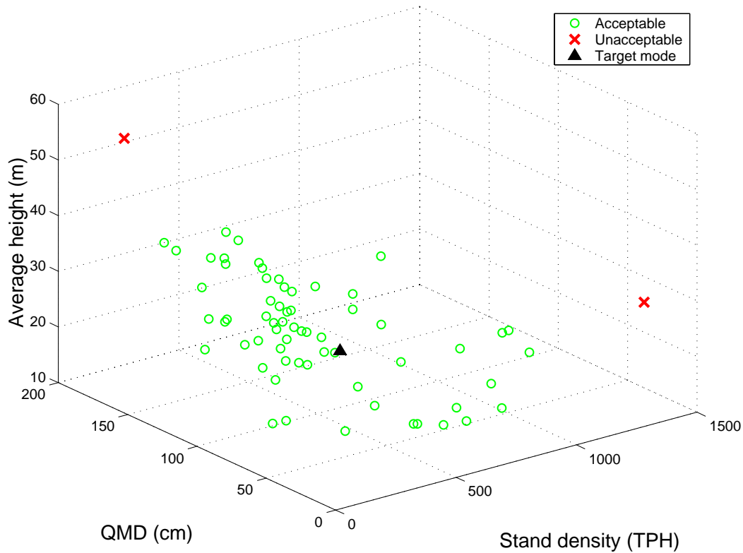
Assessment results: 95% acceptance region about the mode
