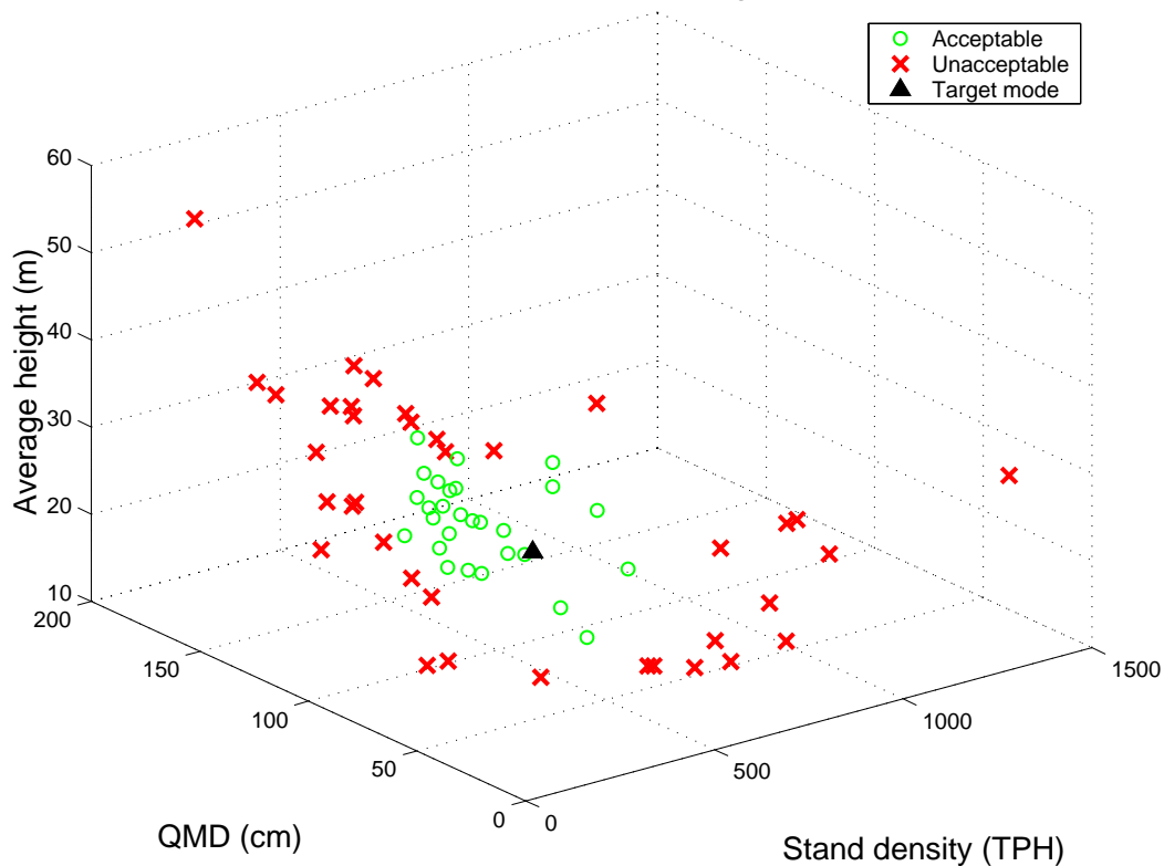
Assessment results: 50% acceptance region about the mode
